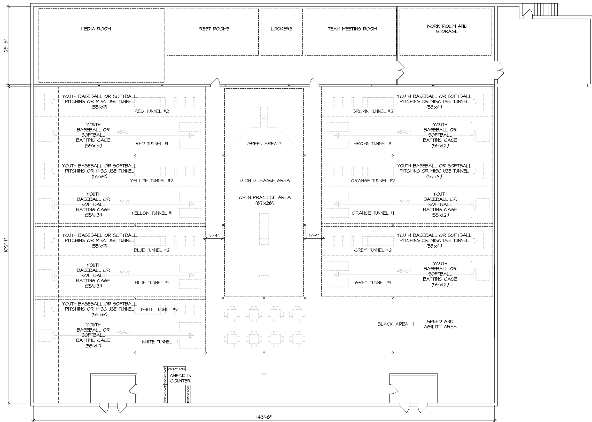
PRELIMINARY LAYOUT
